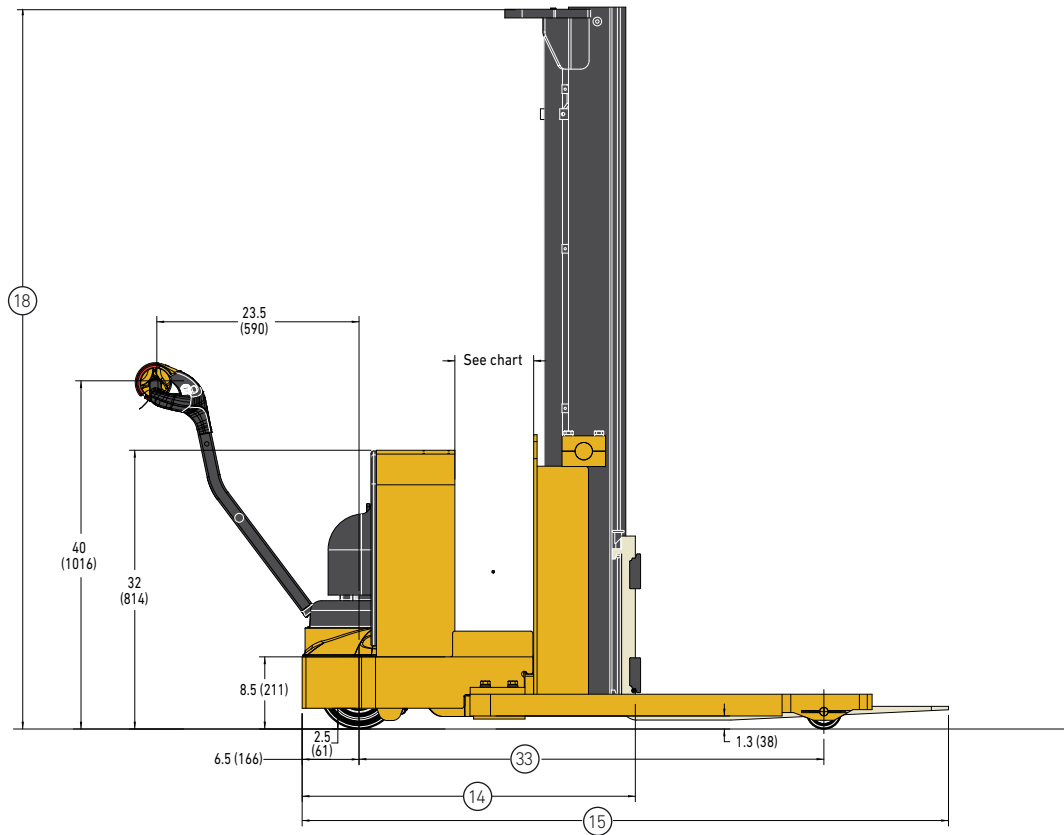
MSW025F Adjustable basearms
